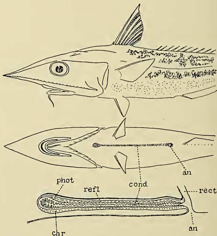
FIG. 3. Diagram of the luminous organ of Coelorhynchus parallelus and its longitudinal section. phot, luminous gland; refl, reflector; cond, conduit; chr, chromatophore; an, anus; rect, rectum.
